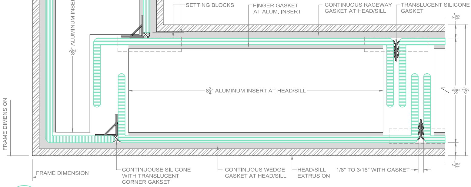
1 TYPICAL CORNER DETAIL SD-4 SCALE: 6" = 1'-0"
