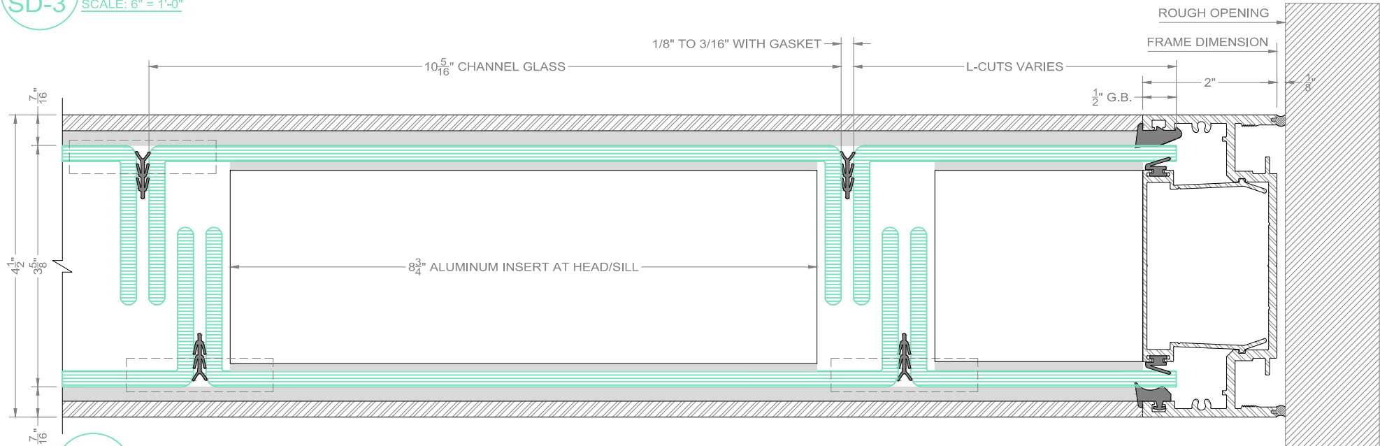
1 JAMB DETAIL AT ADJACENT CONS. WITH L-CUTS SD-3 SCALE: 6" = 1'-0"
